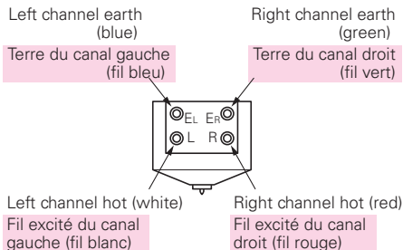
Fig. 2 Arrangement of Output Terminals
