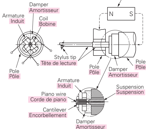
Fig. 6 Moving System Fig. 6 Equipage mobile
